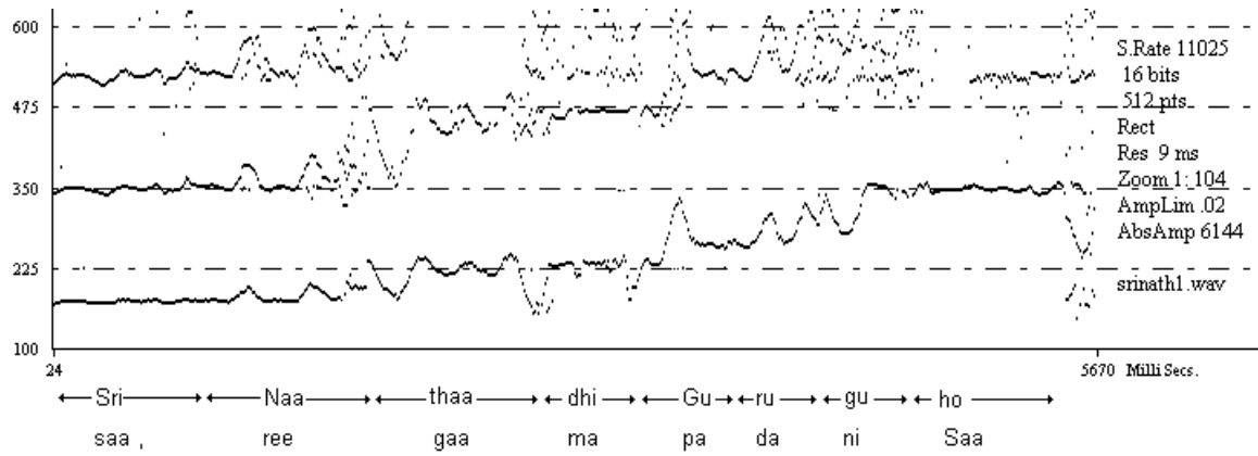
Fig. 1 Part of the first line of Srinaathaadhi Guruguho in Maayamaalavagowla - showing the extensive gamakam.
